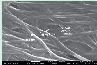
Scanning Electron Microscopy of Nano Skin Membrane
